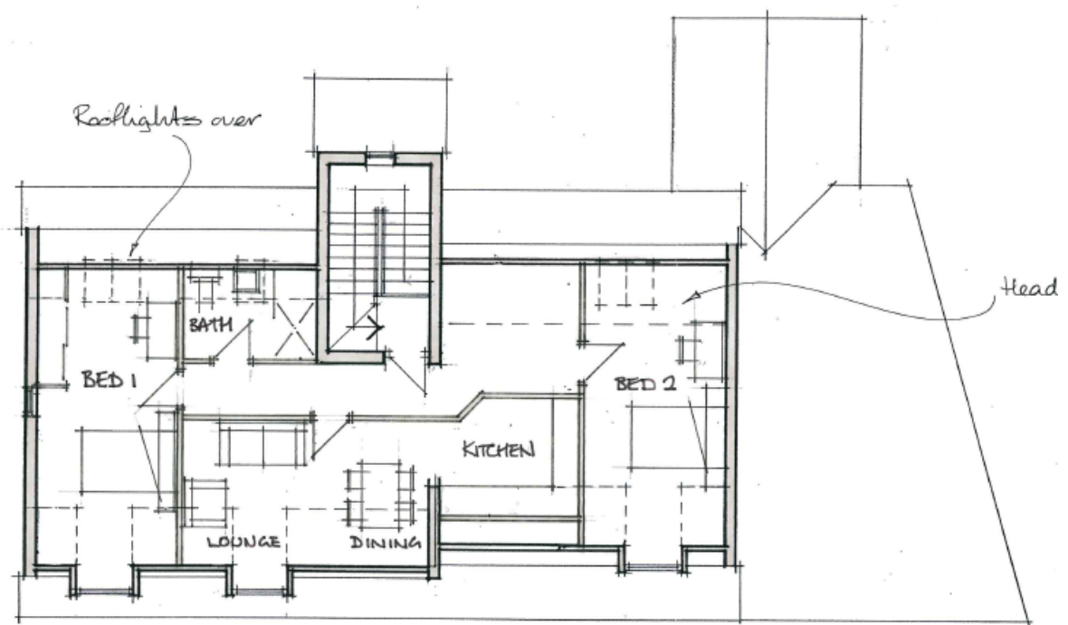
Second floor/roofspace plan
